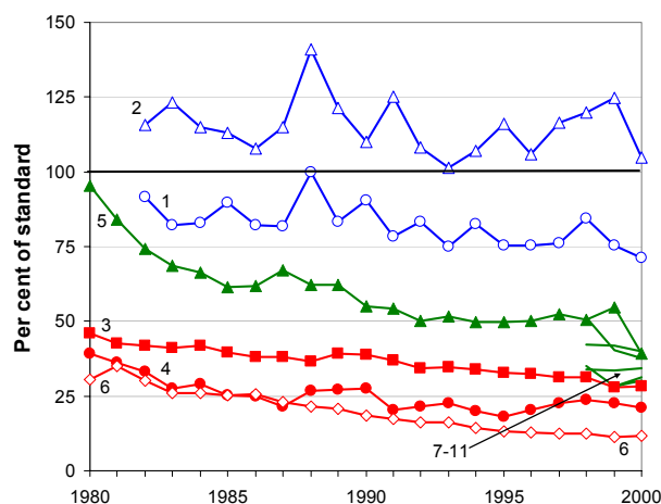
Figure 9. Trends in urban air quality, 1980-2000 (see text for explanation of each of the 11 series)
