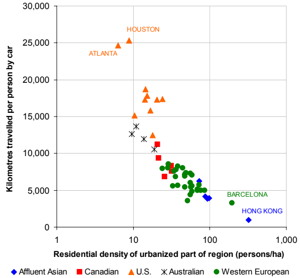
Figure 4. Relationship between urban density and car travel, 52 urban regions, 1995
